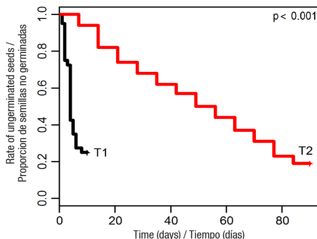
Figure 6. Differences between germination curves, between treatments using the Kaplan-Meier estimator using the R survfit function. T1 = Treatment 1, T2 = Treatment 2.
